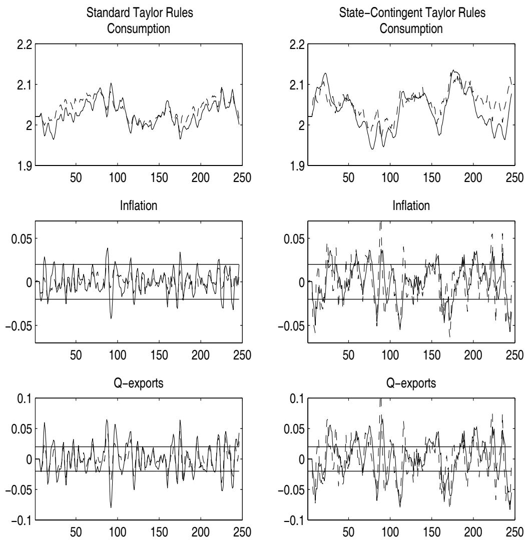
Figure 3: Time Series under Standard and State-Contingent Taylor Rules with Learning: inflation targeting (solid line), inflation/Q-growth targeting (dashed line)
