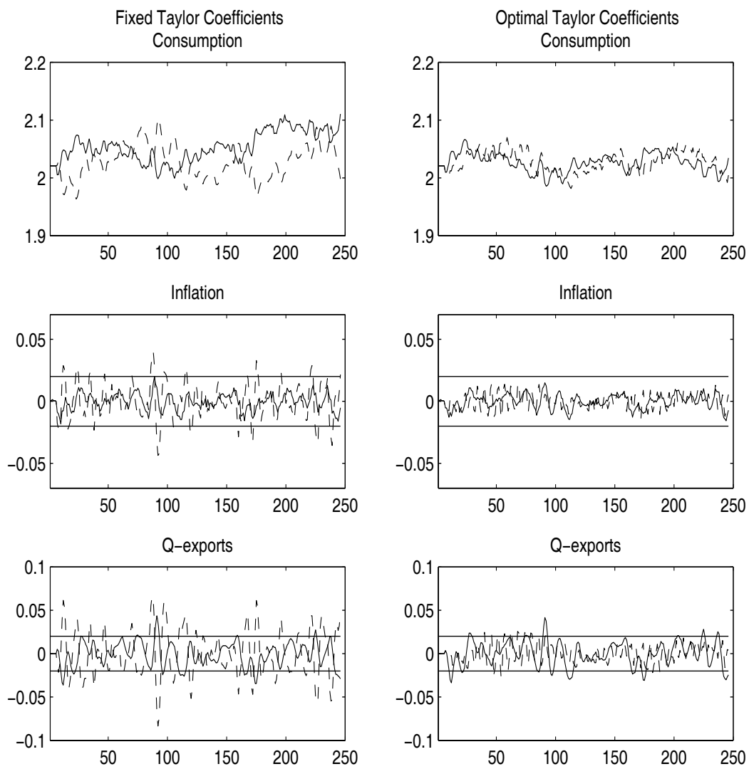
Figure 2: Time Series with Fixed and Optimal Taylor Coefficients with No Learning: inflation targeting (solid line), inflation/Q-growth targeting (dashed line)
