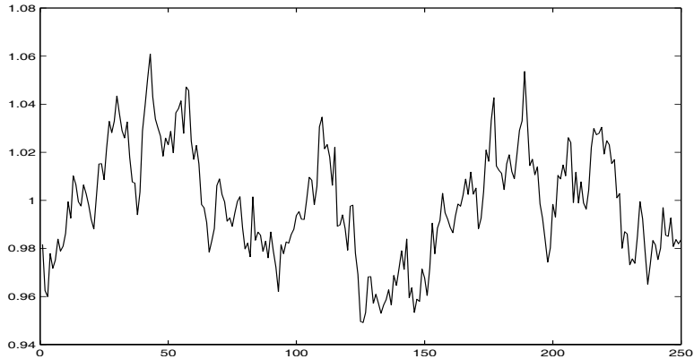
Figure 1: One realization of the terms of trade shocks
